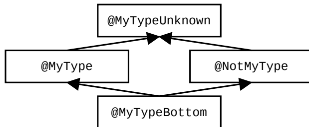
Figure 27.1: Type system for a type alias or typedef type system. The type system designer may choose to omit some of these types, but this is the general case. The type system designer’s choice of defaults affects the interpretation of unannotated code, which affects the guarantees given for unannotated code.
