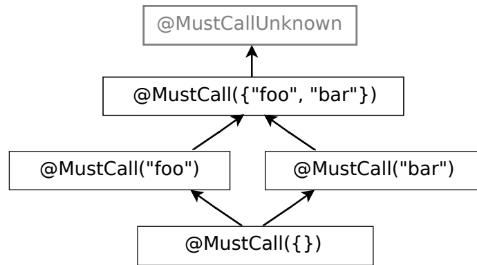
Figure 26.1: Part of the Must Call Checker’s type qualifier hierarchy. The full hierarchy contains one @MustCall annotation for every combination of methods. Qualifiers in gray are used internally by the type system but should never be written by a programmer.
