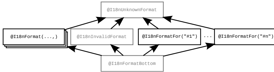
Figure 13.1: The Internationalization Format String Checker type qualifier hierarchy. The type qualifiers are applicable to CharSequence and its subtypes. The figure does not show the subtyping rules among different @I18nFormat(...) qualifiers; see Section 13.2. All @I18nFormatFor annotations are unrelated by subtyping. The qualifiers in gray are used internally by the checker and should never be written by a programmer.
