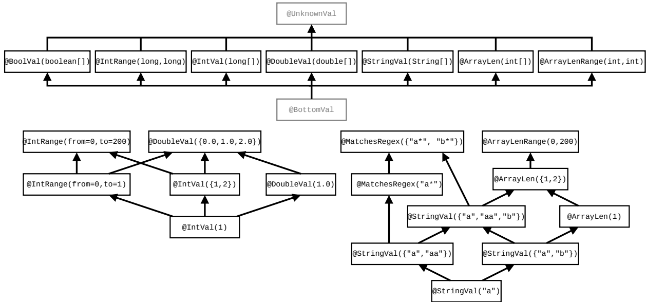
Figure 22.1: At the top, the type qualifier hierarchy of the Constant Value Checker annotations. The first four qualifiers are applicable to primitives and their wrappers; the next to Strings (it can also be written as @EnumVal for enumeration constants), and the final two to arrays. Qualifiers in gray are used internally by the type system but should never be written by a programmer. At the bottom are examples of additional subtyping relationships that depend on the annotations' arguments.
