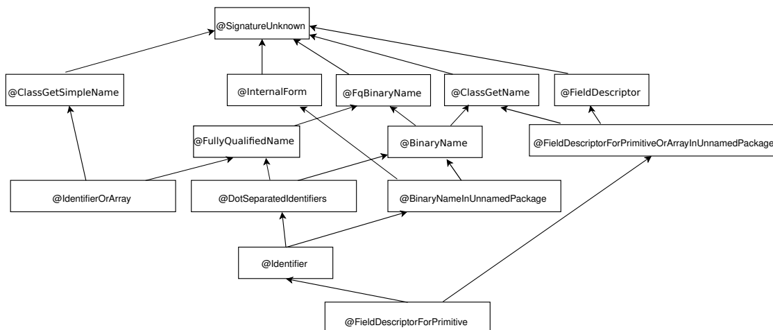
Figure 15.1: Partial type hierarchy for the Signature type system, showing string representations of a Java type. The type qualifiers are applicable to CharSequence and its subtypes. Programmers usually only need to write the boldfaced qualifiers; other qualifiers are included to improve the internal handling of String literals.
