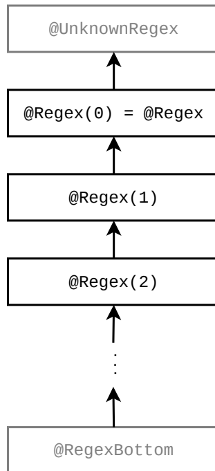
Figure 11.1: The subtyping relationship of the Regex Checker’s qualifiers. The type qualifiers are applicable to CharSequence and its subtypes. Because the parameter to a @Regex qualifier is at least the number of capturing groups in a regular expression, a @Regex qualifier with more capturing groups is a subtype of a @Regex qualifier with fewer capturing groups. Qualifiers in gray are used internally by the type system but should never be written by a programmer.
