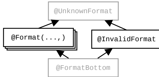
Figure 12.1: The Format String Checker type qualifier hierarchy. The type qualifiers are applicable to CharSequence and its subtypes. The figure does not show the subtyping rules among different @Format(...) qualifiers; see Section 12.2.2.
