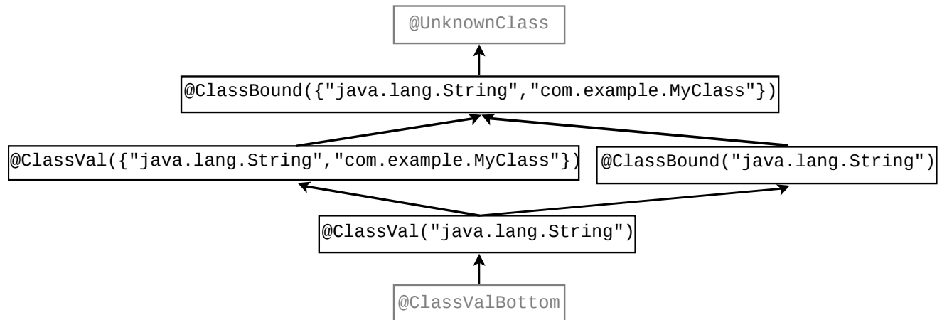
Figure 22.1: Partial type hierarchy for the ClassVal type system. The type qualifiers in gray (@UnknownClass and @ClassValBottom) should never be written in source code; they are used internally by the type system.
