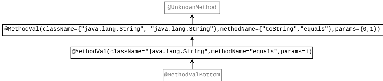
Figure 22.2: Partial type hierarchy for the MethodVal type system. The type qualifiers in gray (@UnknownMethod and @MethodValBottom) should never be written in source code; they are used internally by the type system.
