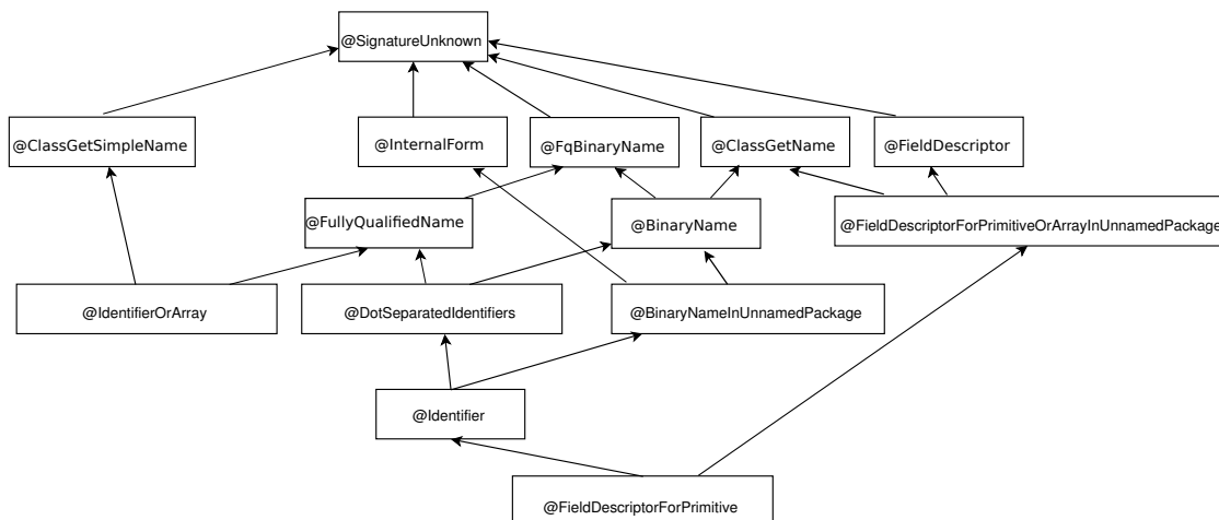
Figure 15.1: Partial type hierarchy for the Signature type system, showing string representations of a Java type. The type qualifiers are applicable to CharSequence and its subtypes. Programmers only need to write the boldfaced qualifiers; other qualifiers are included to improve the internal handling of String literals.
