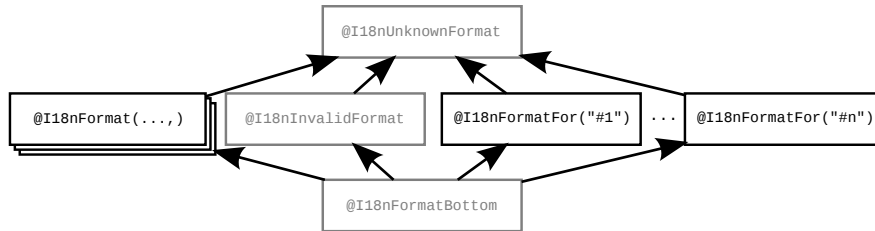
Figure 13.1: The Internationalization Format String Checker type qualifier hierarchy. The type qualifiers are applicable to CharSequence and its subtypes. The figure does not show the subtyping rules among different @I18nFormat(...) qualifiers; see Section 13.2. All @I18nFormatFor annotations are unrelated by subtyping. The qualifiers in gray are used internally by the checker and should never be written by a programmer.
