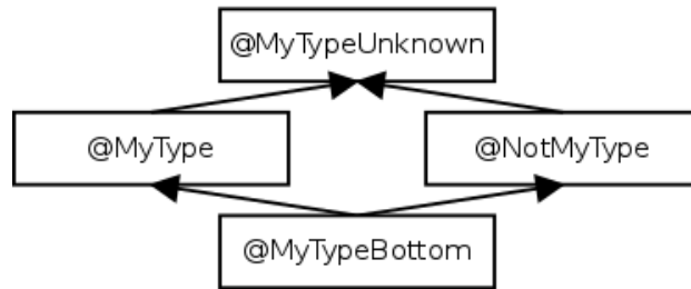
Figure 21.1: Type system for a type alias or typedef type system. The type system designer may choose to omit some of these types, but this is the general case. The type system designer’s choice of defaults affects the interpretation of unannotated code, which affects the guarantees given for unannotated code.
