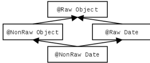
Figure 3.7: Partial type hierarchy for the Rawness Initialization type system.
