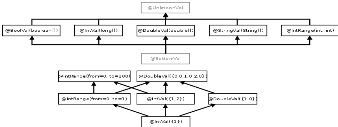
Figure 17.1: At the top, the type qualifier hierarchy of the Constant Value Checker annotations. Qualifiers in gray are used internally by the type system but should never be written by a programmer. At the bottom are examples of additional subtyping relationships that depend on the annotations' arguments.
