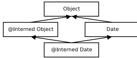
Figure 2: Type hierarchy for the Interning type system.
